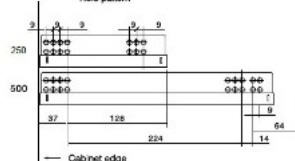
Extension lines
